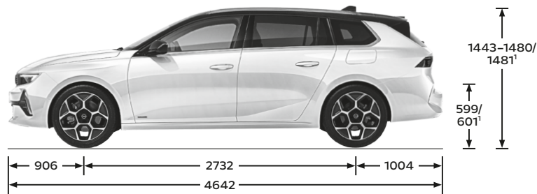
Astra Sports Tourer Alle Masse in mm
